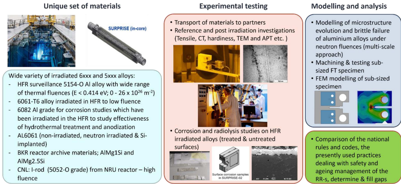
Fig. 2. Methodology applied in Magic-RR project.
