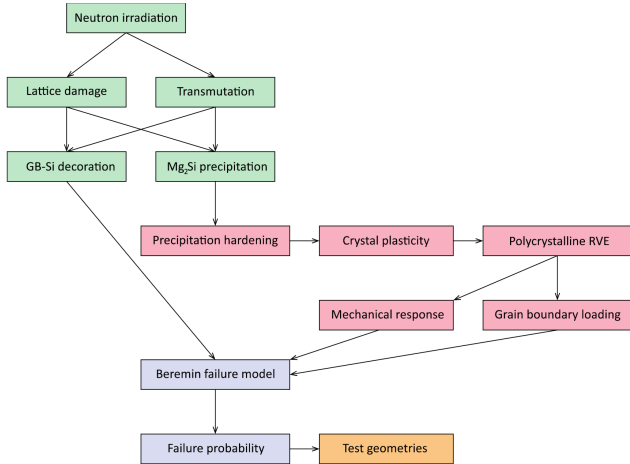
Fig. 4. Modelling of microstructure evolution and brittle failure of aluminum alloys under neutron irradiation.
