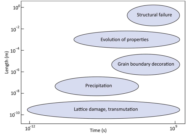
Fig. 5. Length-scales and timescales involved in microstructure evolution and brittle failure of aluminum alloys under neutron fluence.
