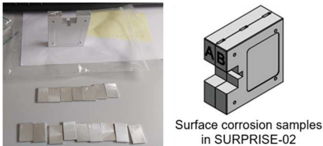
Fig. 3. Picture and drawing of the corrosion specimens irradiated in the SURPRISE irradiation facility of the HFR.
