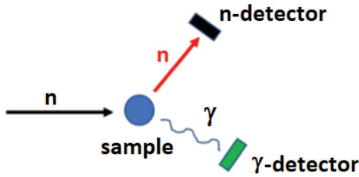
Fig. 1. A basic configuration of measurements related to (n, xn) cross sections. Neutrons from the production target are shown entering from the left. Neutrons and \gamma rays generated by reactions with the sample are recorded by appropriate detectors. The angular dependence of the scattering is recorded by rotating the detectors about the center of the sample in the scattering plane or by using a multiple-detector array.
