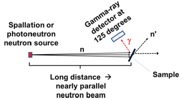
Fig. 6. Schematic representation of neutron scattering experiments at a white neutron source where only the \gamma rays are detected.
