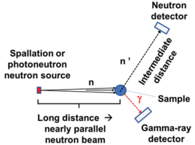
Fig. 9. Schematic representation of neutron scattering experiments at a white neutron source lab where the scattered neutrons and \gamma rays are both detected.
