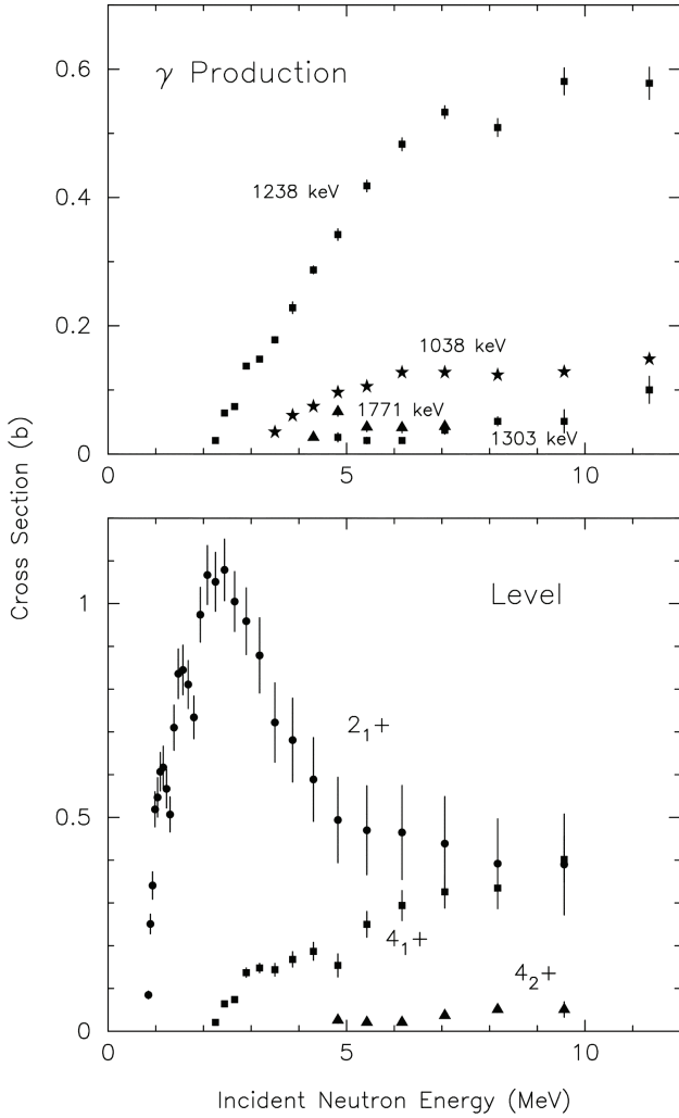
Fig. 8. Representative ^{56}\text{Fe} results employing \gamma -ray detection following inelastic neutron scattering from the (n, n'\gamma) reaction at the white-source laboratory nELBE to extract level cross sections over a wide range of energies. \gamma -ray production cross sections are measured (top) and feeding is subtracted to extract level cross sections (bottom) [21]. Other good examples are the ^{56}\text{Fe}(n, n'\gamma) data of Negret [15] and the ^{23}\text{Na}(n, n'\gamma) data of Rouki [16] taken at GELINA.
