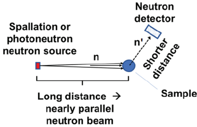
Fig. 4. Schematic representation of neutron scattering experiments at a white neutron source facilities where only the scattered neutrons are detected.
