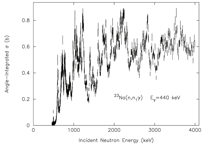
Fig. 7. Representative cross sections employing \gamma -ray detection following the ^{23}\text{Na}(n, n'\gamma) reaction at the white-source laboratory GELINA to extract level cross sections with fine energy resolution in the resonance region [16].
