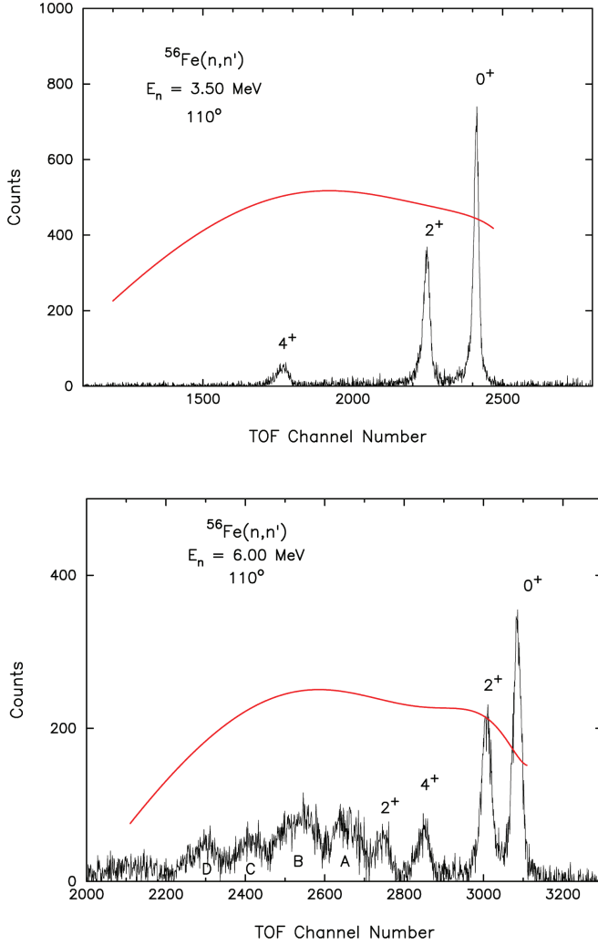
Fig. 3. Representative background-subtracted neutron TOF spectra of ^{56}\text{Fe}(n, n') typical of Van de Graaff laboratories; these data are published in reference [37]. Peaks are labeled with the residual nucleus spin. The red line is an example of the energy-dependent neutron detector efficiency, here displayed as a function of channel number. These spectra illustrate the difficulties encountered in TOF measurements, where typically only scattering from a few low-lying states can be resolved. Clumps of levels (A-D) develop at higher energies and although one knows the levels in each clump from nuclear structure investigations, it is generally not possible to extract the individual contributions. For low mass targets, say A < 40 , multiple scattering in the sample creates left-side, lower energy tails and features that make it difficult to extract the yields of neighboring peaks.
