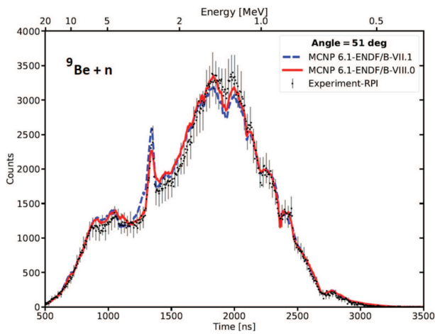
Fig. 5. Representative spectrum from neutron scattering measurements on beryllium at RPI that is typical of white neutron source laboratories. The raw measurements are overlaid with MCNP simulations of the experiment geometry [41]. The experimental setup and additional details of neutron scattering measurements at RPI can be found in reference [101].
