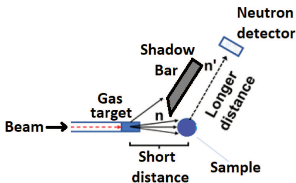
Fig. 2. Schematic representation of neutron scattering experiments with monoenergetic neutron sources where only the scattered neutrons are detected. The shadow bar blocks the detector from seeing source neutrons directly. An advanced shadow bar construction is described in reference [34]. Measurements are made with sample-in and sample-out.
