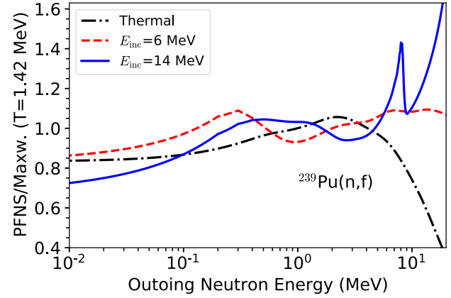
Fig. 3. ENDF/B-VIII.0 ^{239}\text{Pu} PFNS [8,60] are used as examples to illustrate structures commonly observed around second- and third-chance fission thresholds: from thermal E_{\text{inc}} to the on-set of second chance fission, curves similar in shape to the thermal PFNS are expected. In a window of E_{\text{inc}} = 1\text{--}2 MeV around second-chance fission (red dashed line), one sees a characteristic structure of the PFNS appear in the 100s of keV stemming from a second-chance fission contribution to the PFNS that is only non-zero up to these energies due to energy conservation. Around the third-chance fission threshold (blue solid line), this structure is like a broader shoulder in E_{\text{out}} above 100 keV. One also sees a sharp structure at high E_{\text{out}} (several MeV) coming from the pre-equilibrium neutron emission from the compound nucleus before fission happens.
