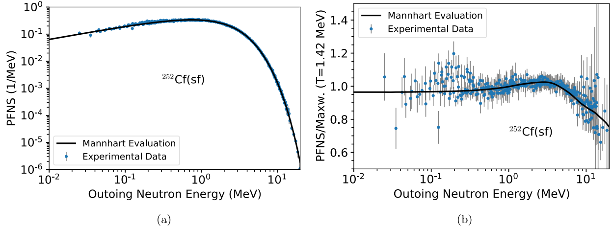
Fig. 1. The evaluated ^{252}\text{Cf} spontaneous fission spectrum by Mannhart [2,3] is compared to the experimental data used for that evaluation and as shown in Figures 1–10 of reference [2]. (a) The PFNS in units of (1/\text{MeV}) . (b) The PFNS as a ratio to a Maxwellian function.
