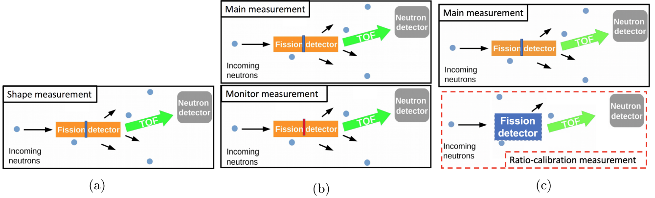
Fig. 2. Schematic drawing of PFNS-measurement types. The blue rectangle in the orange fission chamber is the isotope investigated; the blue circles indicate neutrons, including the incident neutron, and scattered or background neutrons; the green arrow denotes fission neutrons headed to the neutron detector; other fission neutrons are given by the black arrows. Figure (a) is for shape measurements. Figures (b) show the main measurement (top) and the monitor measurement (bottom) for a clean-ratio shape measurements. Figures (c) show the main measurement (top) and an associated ratio-calibration measurement (bottom) made in a different experimental environment to quantify the neutron detector efficiency. Figure 3 (c-bottom) can also illustrate calibration with a spontaneous fission source such as ^{252}\text{Cf} .
