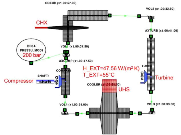
Fig. 7. Layout of the sCO 2 loop modeled with CATHARE 3.
