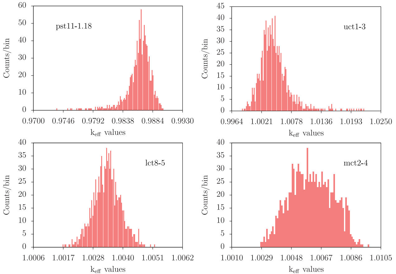
Fig. 1. Probability density function for a number of criticality benchmarks, obtained by randomly changing the H in H 2 O thermal scattering data.
