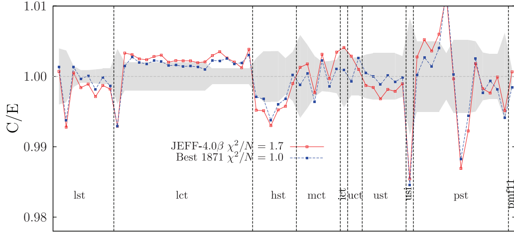
Fig. 3. Calculated over Experimental values for the considered criticality benchmarks. The case “Best” corresponds to a selected H in H 2 O thermal scattering data case.
