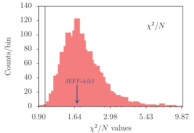
Fig. 2. Distribution of the \chi^2 per degree of freedom considering sampled (random) H in H 2 O thermal scattering data. The vertical black line indicates the position of \chi^2/N = 1 .
